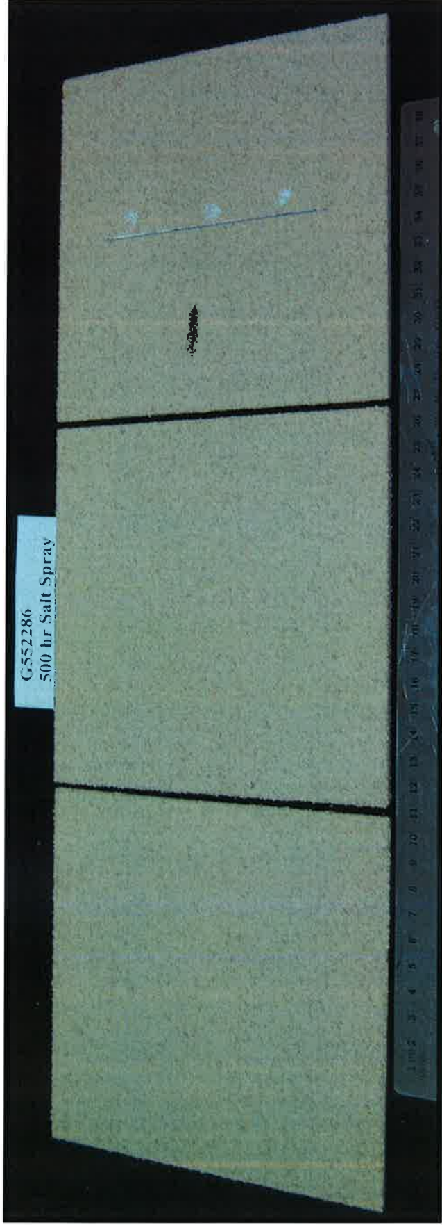
Figure 2: Photograph illustrating the specimens after 500 hours of salt spray exposure. The specimens showed slight softening with no blistering, lifting, loss of adhesion or other visible changes. There was no loss of adhesion/creepback from the scribe.
